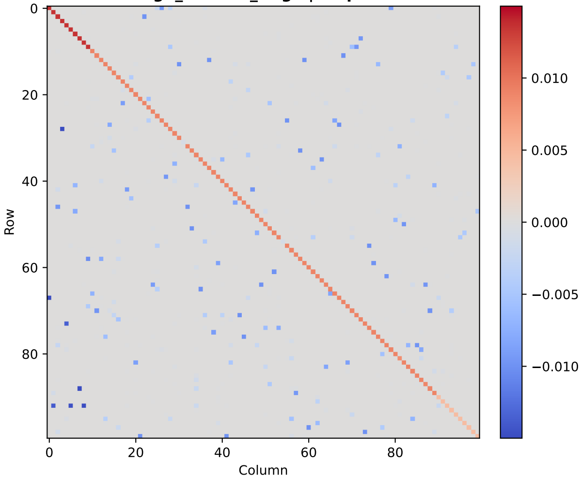
gd_random_large | step 2
